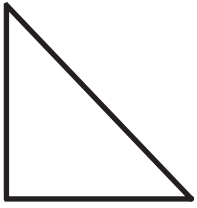
right triangle
