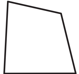
trapezoid
