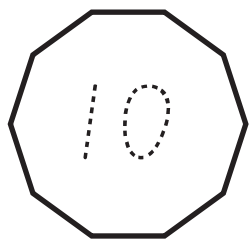
decagon
